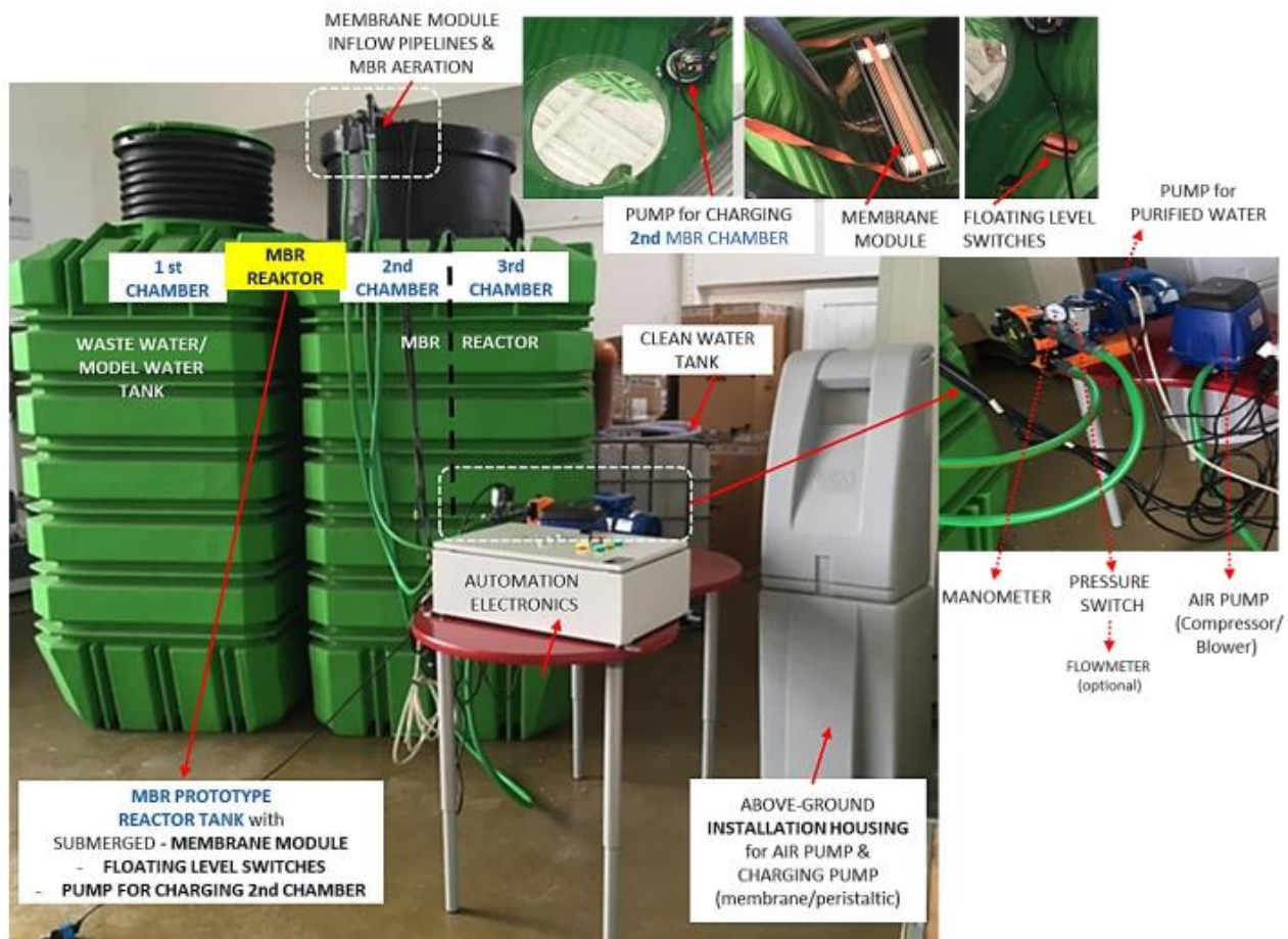
Figure 1. Composition of the EQUIPPED PROTOTYPE MBR REACTOR ( V=6\text{ m}^3 ) with 3 chambers
